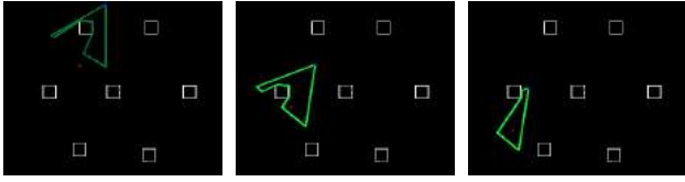
Fig. 3: 2D simulation process illustrating the pursuer’s progression from initial discovery to stable tracking, Light green and bright green indicate successful tracking, signifying that, at that moment, the signed distance from the evader to the pursuer’s visible region is less than zero.
